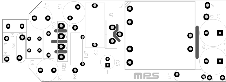
Figure 2 - Top Layer
