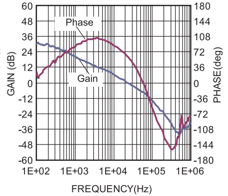
Bode Plot
