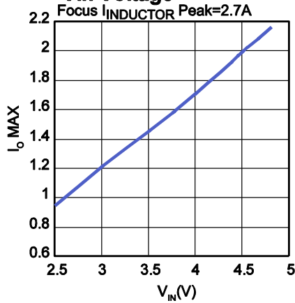
Max. Output Current Vs. Vin Voltage
