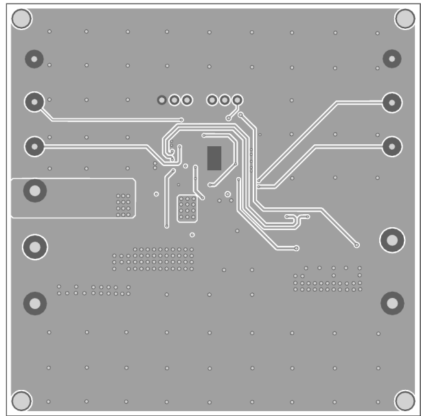
Figure 4—Inner Layer 2
