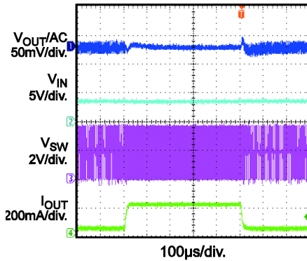
Load Transient I_{OUT} = 30-200mA , 0.25A/\mu s
