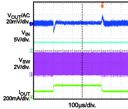
Load Transient I_{OUT} = 100-200mA , 0.25A/\mu s
