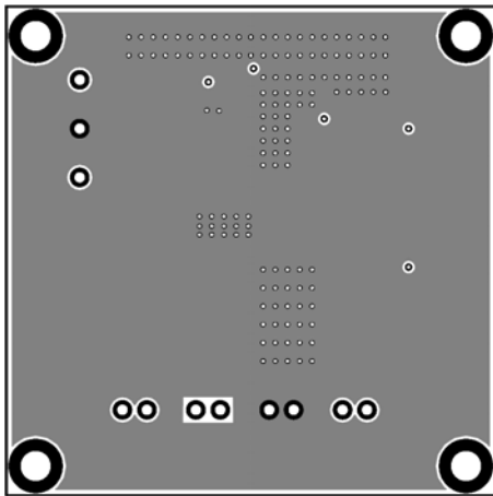
Figure 3—Inner Layer 1
