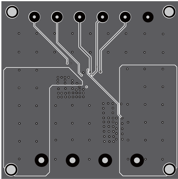
Figure 3—Inner Layer 2
