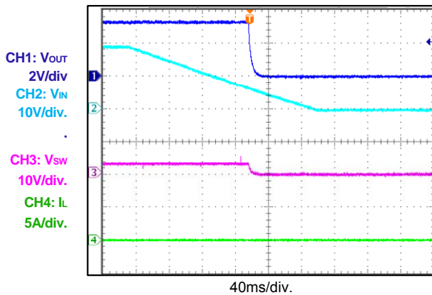
Shutdown through Input Voltage I_{OUT} = 0A
