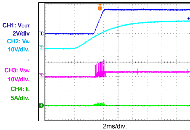
Startup through Input Voltage I_{OUT} = 0A
