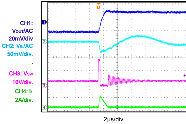
Input/Output Ripple I_{OUT} = 0A
