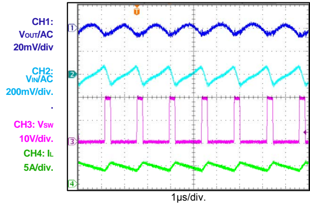
Input/Output Ripple I_{OUT} = 4A
