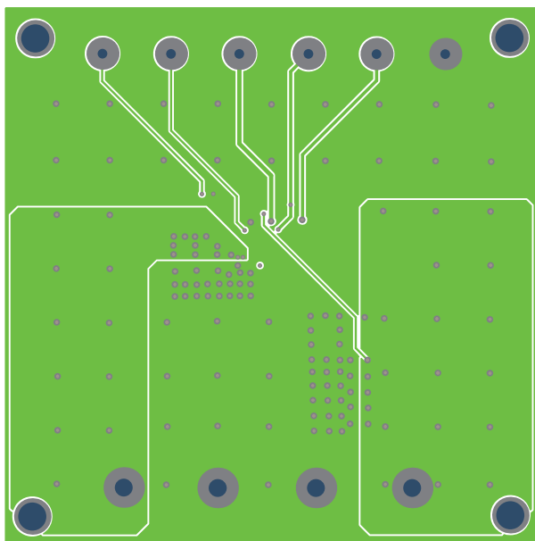
Figure 3—Inner Layer 2
