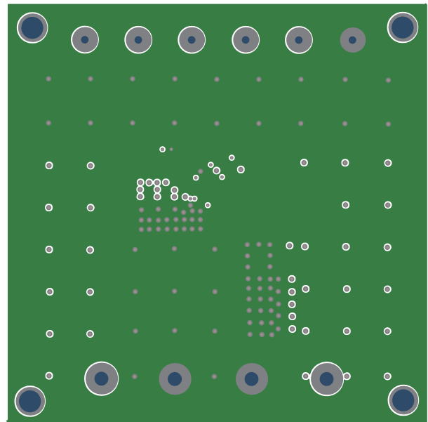
Figure 2—Inner Layer 1
