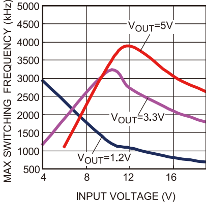
Max Frequency vs. Input Voltage
