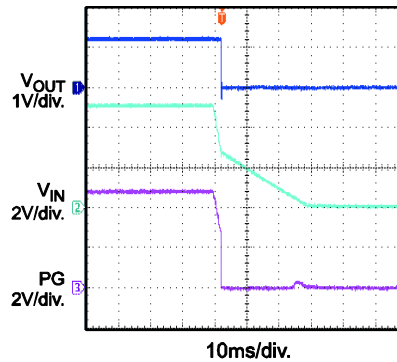
Power Good Through Shutdown
