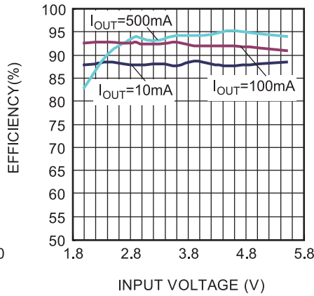
Efficiency vs. Input Voltage MODE=LOW
