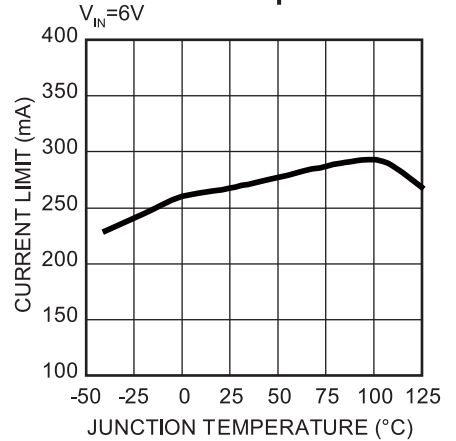
Current Limit vs. Junction Temperature V_{IN} = 6V
