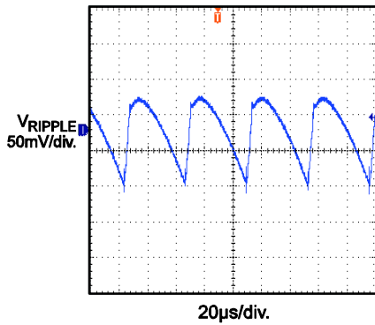
Output Ripple V_{IN} = 115\text{VAC} , Full Load
