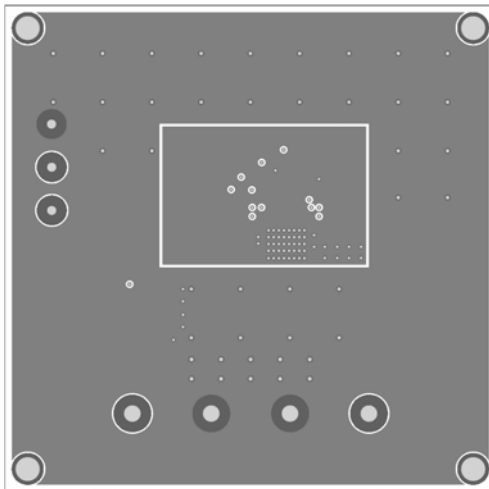
Figure 3—Inner1 Layer
