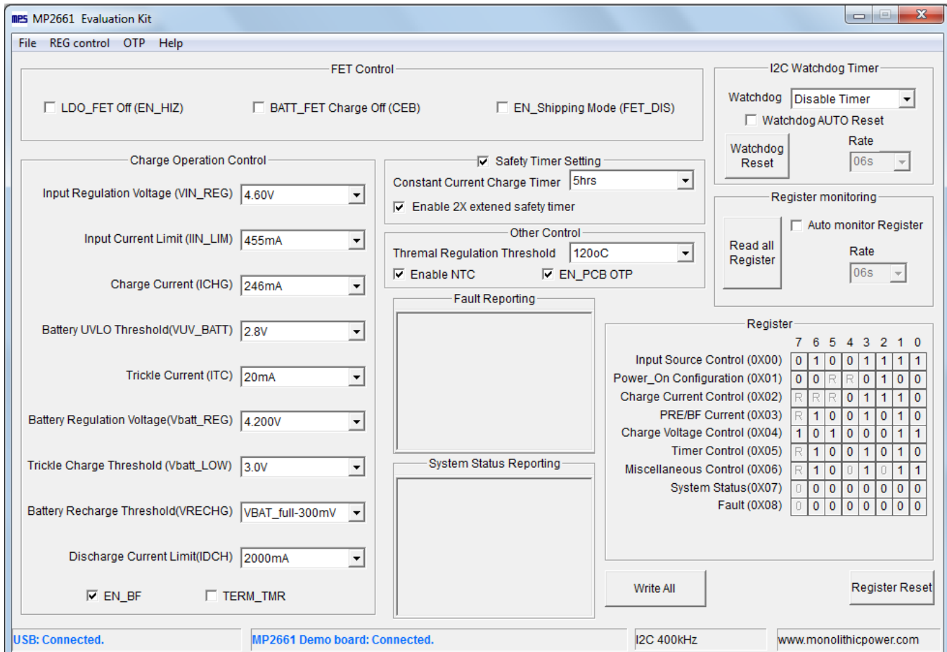
Figure 7: Appearance of USB and MP2661 EVB Board Show Connected
