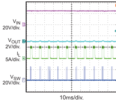
Short Circuit Recovery I_{OUT} = 3A
