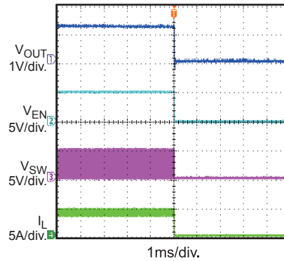
Enable Shutdown I_{OUT} = 4A , PFM
