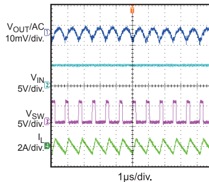
Steady State No Load, PWM
