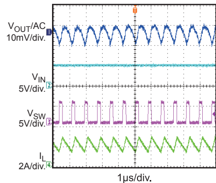
Steady State Half Load 2A, PWM
