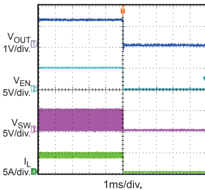
Enable Shutdown I_{OUT} = 4A , PWM
