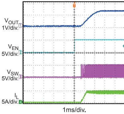
Enable On I_{OUT} = 4A , PFM
