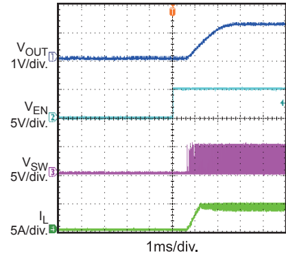
Enable On I_{OUT} = 4A , PWM
