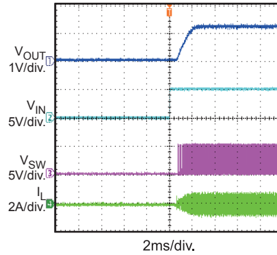
Enable On I_{OUT} = 0A , PWM
