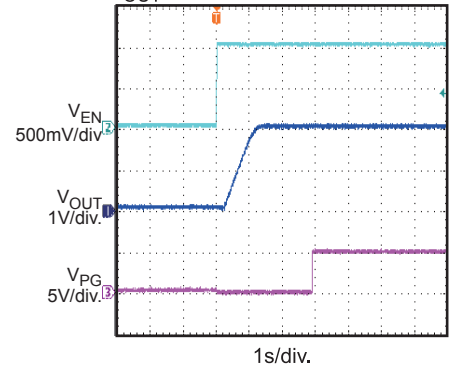
Power Good through EN Start Up I_{OUT} = 0.5A
