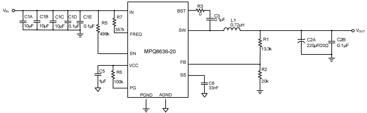
Figure 10 — Typical Application Circuit with No External Ramp MPQ8636-20, V_{IN} =12V, V_{OUT} =1V, I_{OUT} =20A, f_{SW} =500kHz
