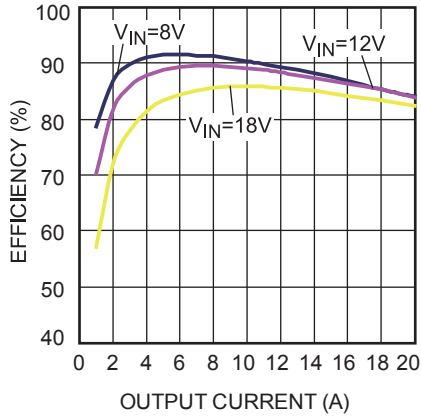
Efficiency vs. Output Current @500kHz
