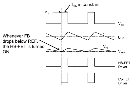
Figure 2: PWM Operation
