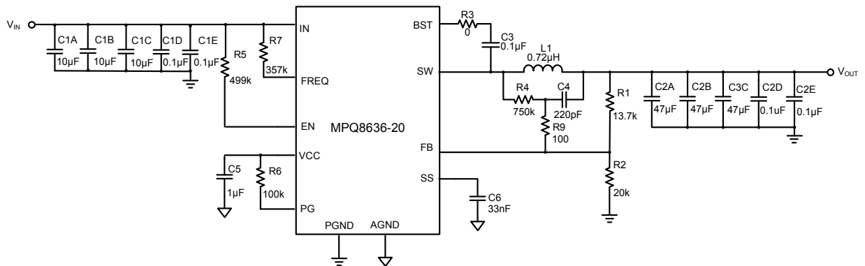
Figure 11 — Typical Application Circuit with Low ESR Ceramic Capacitor MPQ8636-20, V_{IN} =12V, V_{OUT} =1V, I_{OUT} =20A, f_{SW} =500kHz
