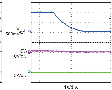
Thermal Shutdown I_{OUT} = 0A
