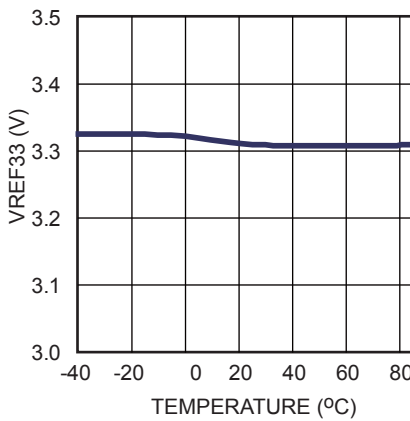
VREF33 vs. Temperature
