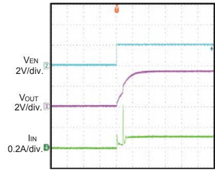
Inrush Current
