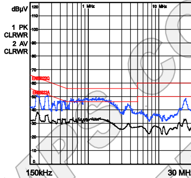
EMI Three Line, 110V, N
