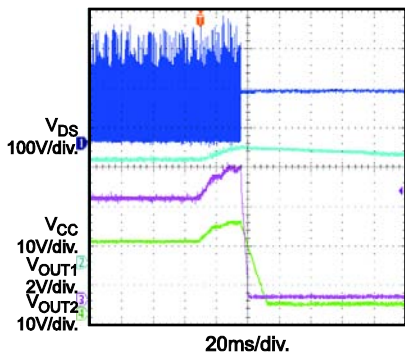
OVP V_{IN}=90V_{AC}
