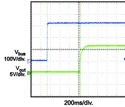
Turn on Delay V_{IN} = 230Vac No load
