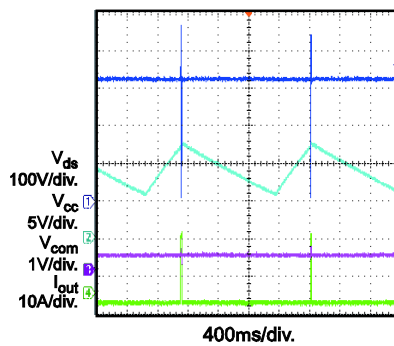
Protection V_{IN} = 230Vac short circuit protection
