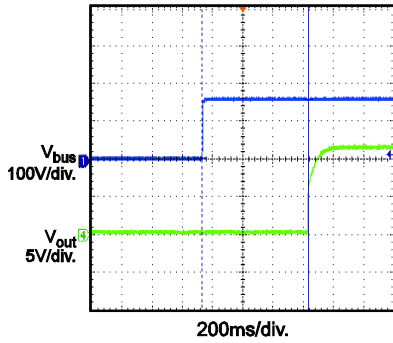
Turn on Delay V_{IN} = 115Vac No load
