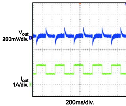
Load Transient V_{IN} = 115Vac 25% to 50%
