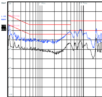
Conducted EMI two line 115Vac
