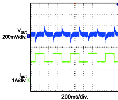
Load Transien V_{IN} = 230Vac 50% to 75%
