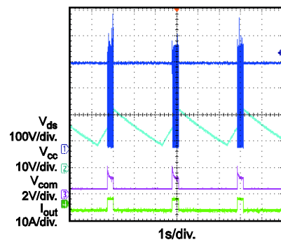
Protection V_{IN} = 230Vac Over load protection
