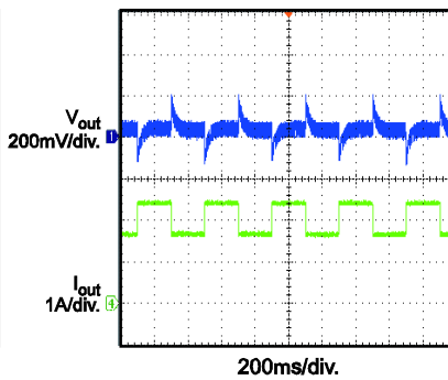
Load Transient V_{IN} = 115Vac 50% to 75%
