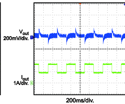
Load transient V_{IN} = 230Vac 25% to 50%
