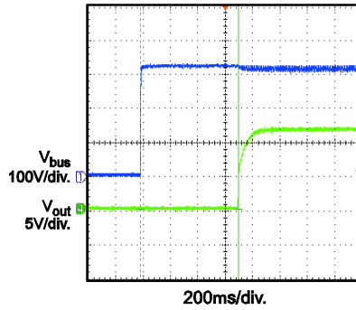
Turn on Delay V_{IN} = 230Vac Full load
